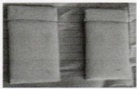
Fig. No. 1 TLC of isolated compound
