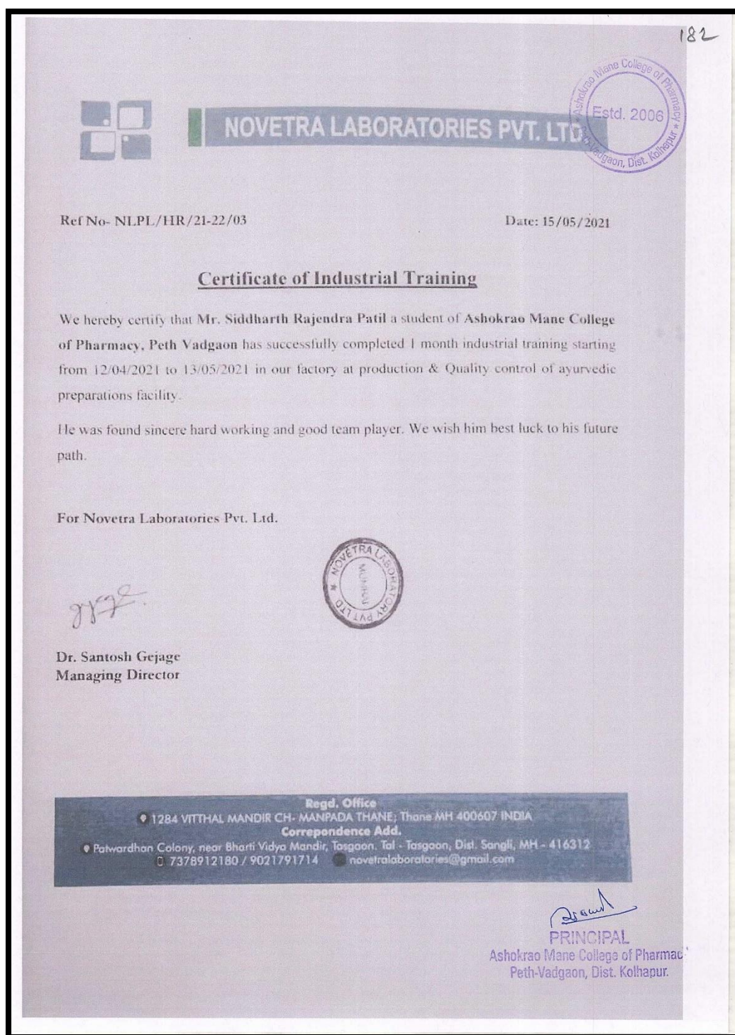
Certificate of Industrial Training No.2
